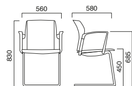
CLASS 100 CANTILEVER WITH ARMS
