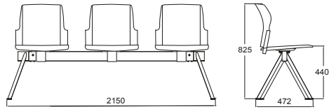
CLASS 100 V LEGS BENCH
