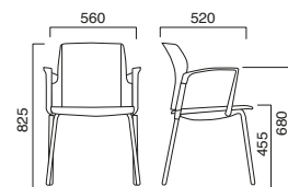
CLASS 100 4 LEGS WITH ARMS
