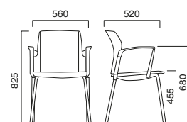
CLASS 100 4 LEGS WITH ARMS FOR UPHOLSTERY
