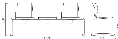
CLASS 100 T LEGS BENCH
