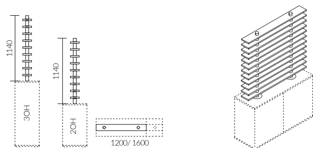
Diviso 3OH with two poles - affixed to top of the cabinet 2/3OH
