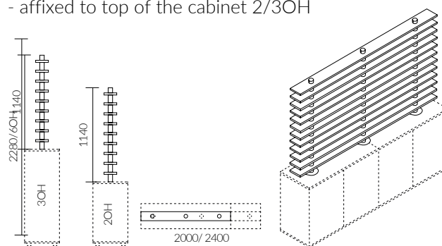
Diviso 3OH with three poles - affixed to top of the cabinet 2/3OH
