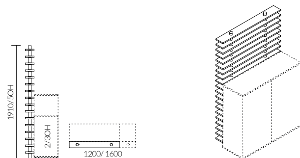
Diviso 5OH with two poles - affixed to back wall of the cabinet
