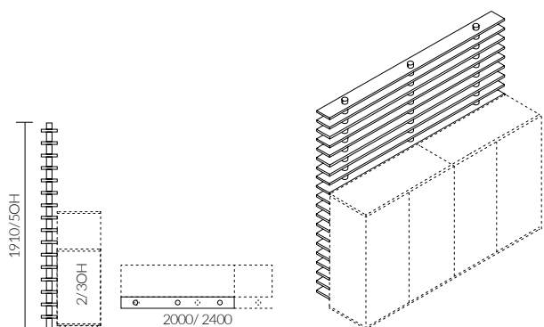
Diviso 5OH with three poles - affixed to back wall of the cabinet
