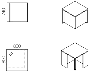
Low corner reception counter H: 740 mm
