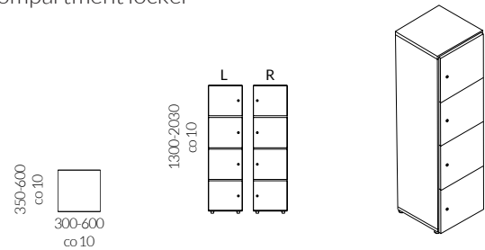
4-compartment locker
