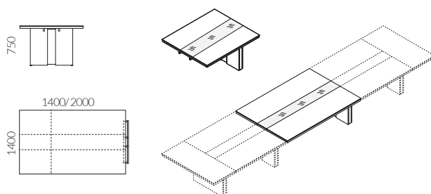
Extension for Ario two-piece conference table with glass insert
