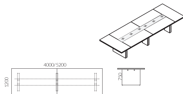
Ario two-piece conference table with glass insert
