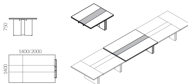
Extension for Ario two-piece conference table with board insert
