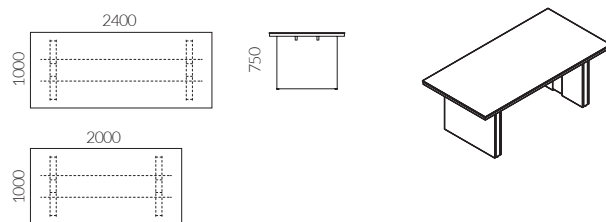
Ario one-piece conference table
