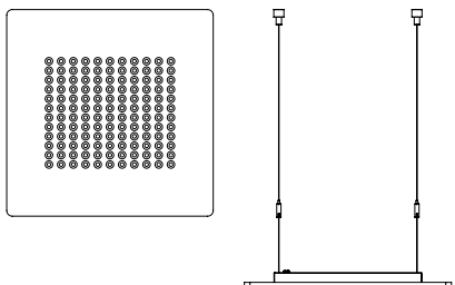
Silurus–Ply lamp 400 × 400 × max. 900 mm (L×W×H)
