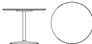
MOTHERSHIP large round tea table w/ metal base Ø900 × 737 mm (D × H)
