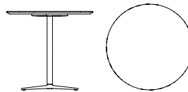
MOTHERSHIP round tea table w/ metal base Ø800 × 737 mm (D × H)
