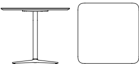
MOTHERSHIP large square tea table w/ metal base 800 × 800 × 737 mm (L × W × H)
