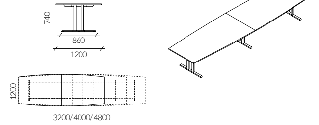
Two-piece conference table with barrel-shaped top
