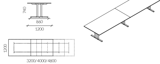
Two-piece conference table with rectangular top
