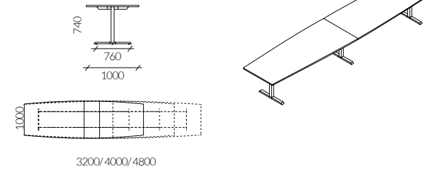
Two-piece conference table with barrel-shaped top
