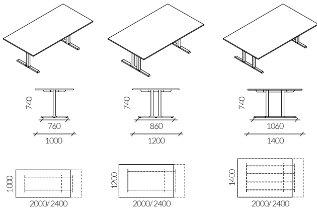
Conference table with rectangular top
