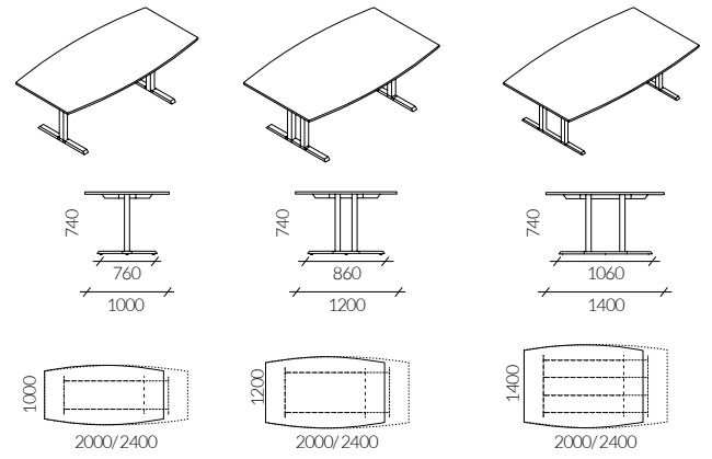
Conference table with barrel-shaped top
