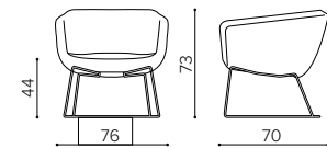
AA 7095 base a slitta • sled base
