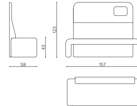
OR B000 panca • bench
