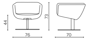
AA 709P base a piastra • plate base
