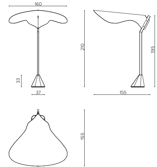
CAP ombrello acustico • acoustic umbrella
